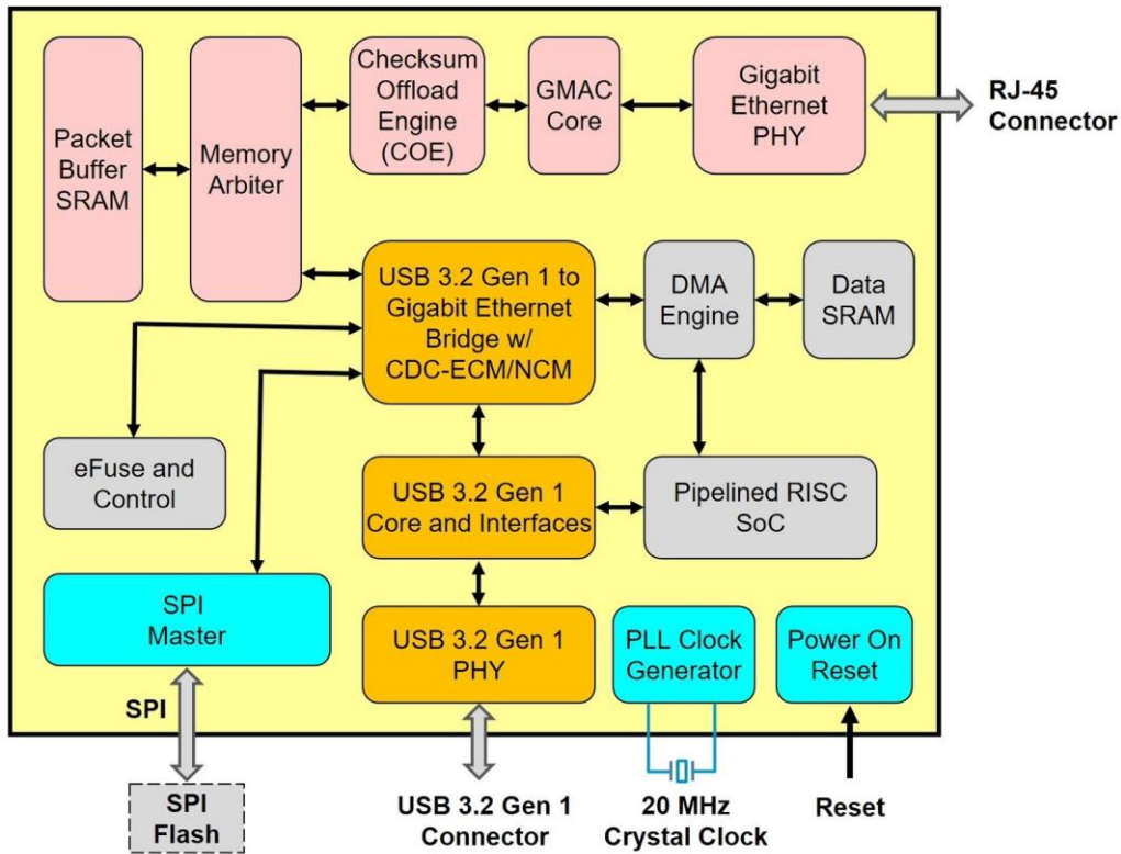
Figure 1-1: AX88179B Block Diagram
